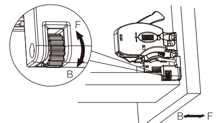
Depth (In and Out) adjustment 0 ~ +3mm
